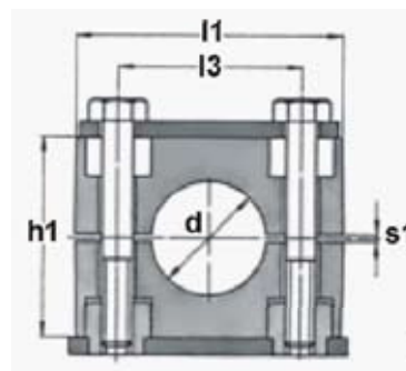
Size 01 to 08
