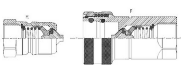
ISO 7241-1B-Strd. 19.02
