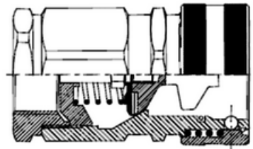
Muffe / female
