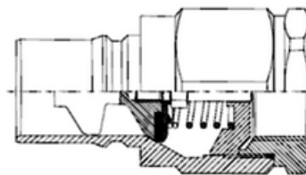
Muffe / female
