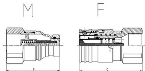
ISO 16028-Strd. 19.06
