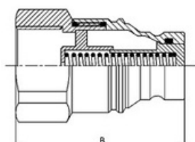
Muffe / female
